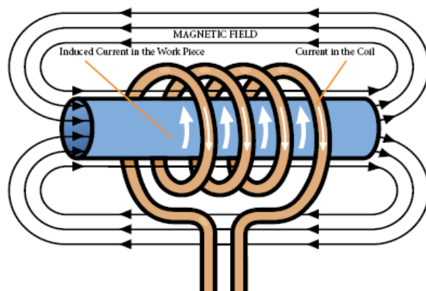
Fig. 1: The principle of single-sided heating.
